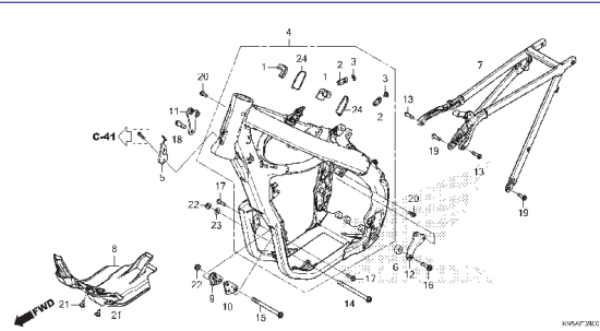
C-39 Chassi
